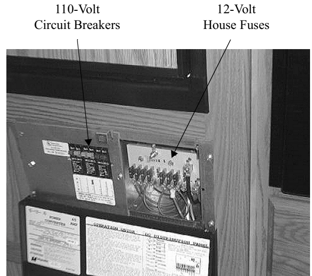
Power Converter
