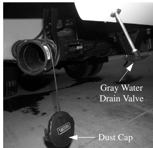
Gray Water Sewage Drain Outlet (Located behind the driver rear wheel)
