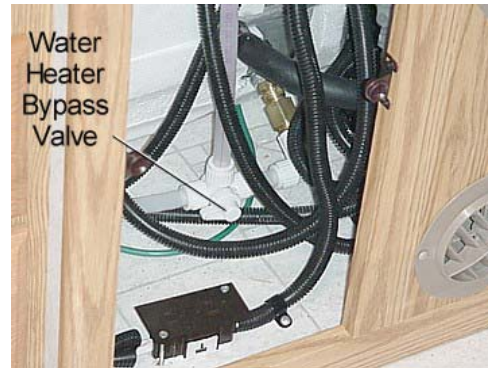
Typical Installation
