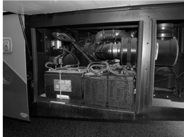
Chassis and House Batteries (Located in rear driver side compartment) -Typical installation shown
