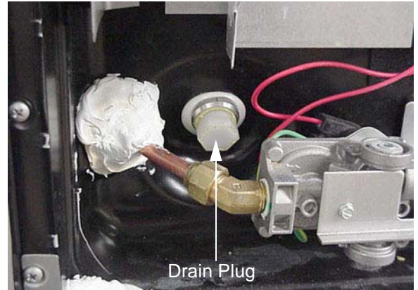
Water Heater Service Access -Typical View
