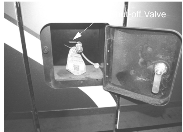
LP Accessory Connection (Located behind lockable access door on passenger side of coach) -Typical View
