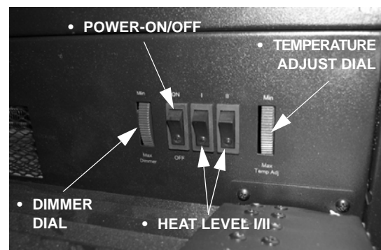
Fireplace Operation Control (Located behind front grill)
