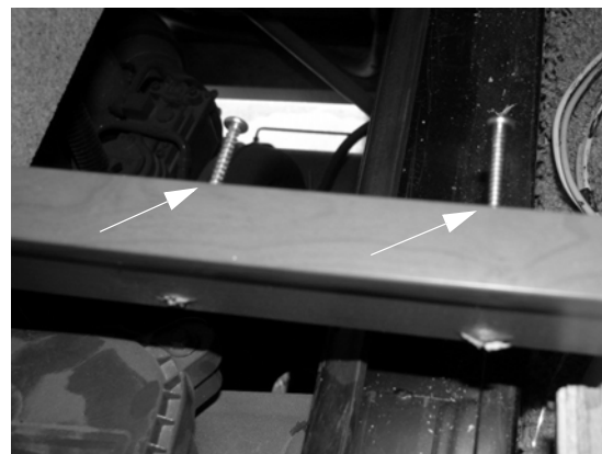
Remove two screws attaching bed board frame to step cover -Typical installation shown
