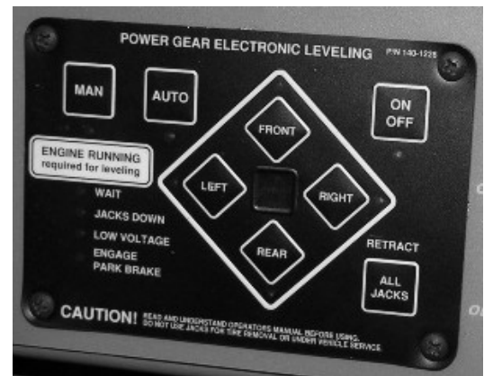
Leveling System Control Panel
