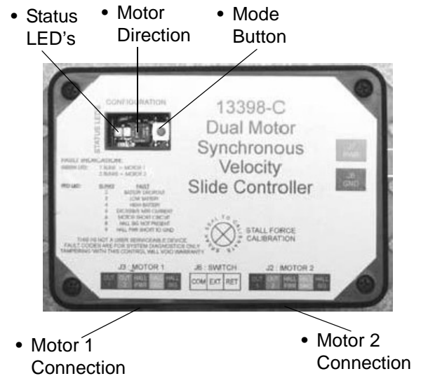
Slideout Control Panel (Located in driver side compartment)
