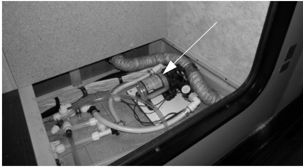
Water Pump (Located beneath removable access panel in passenger rear compartment) -Model 24M shown
