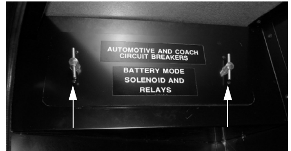
Chassis and House 12V Breaker Panel (Located in passenger side compartment) -Turn both latches to remove cover
