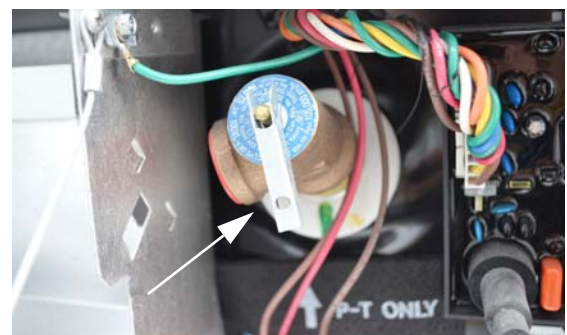
Pressure-Temperature Relief Valve (Lift handle only when water heater is cold)
