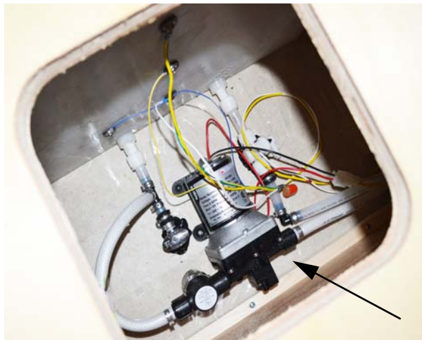
Water Pump (Located beneath bed - lift mattress to expose access hole) -Typical View
