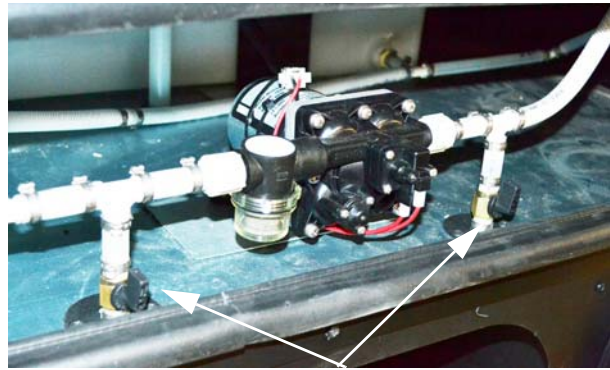
Waterline Drain Valves (Located in second driver side compartment) *Model 34T shown
