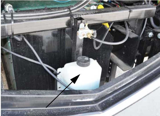
Windshield Washer Reservoir (Located behind front hood panel) -Typical installation shown
