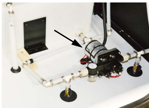
Water Pump (Located in driver side front compartment) -Typical installation shown
