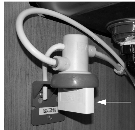
Diverter Plug
