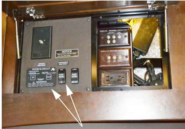
Front Slideout Switches (Your coach may have one or more of these switches depending on model, options, and available equipment) -Typical View
