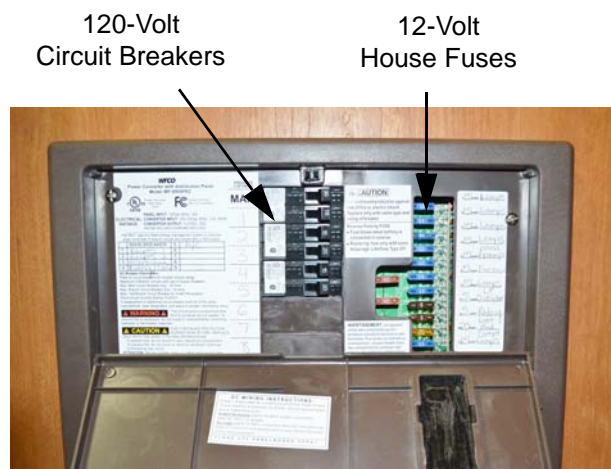
Power Center (Models 27N and 30T) -Typical View
