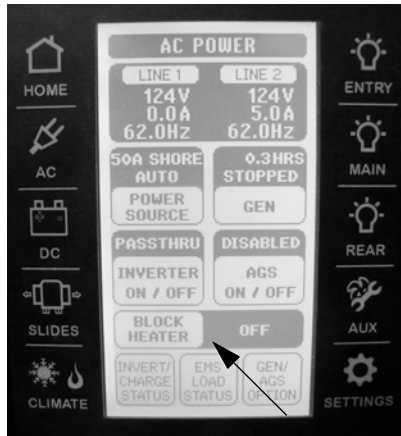
Diesel Engine Heater Switch (Located on multiplex monitor panel)
