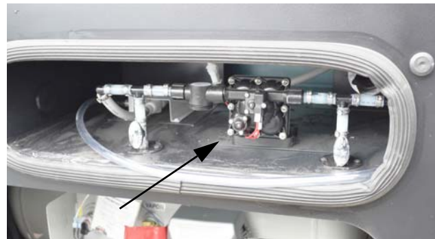
Water Pump (Located in driver side front compartment) -Typical installation shown
