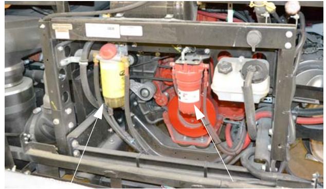
Diesel Fuel/Water Separator (Filter)
