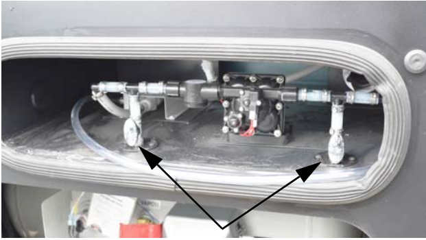
Waterline Drain Valves (Located in driver side compartment) -Typical installation shown
