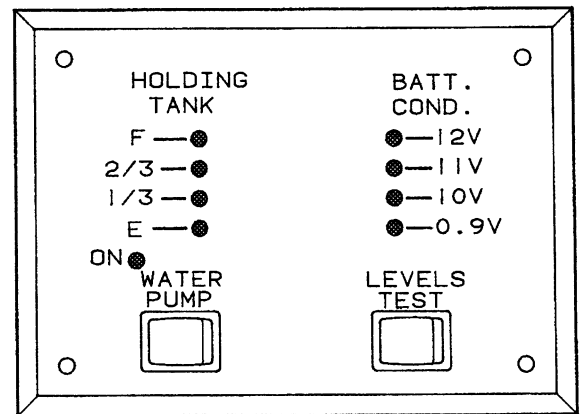
Monitor Panel - Model 23RC
