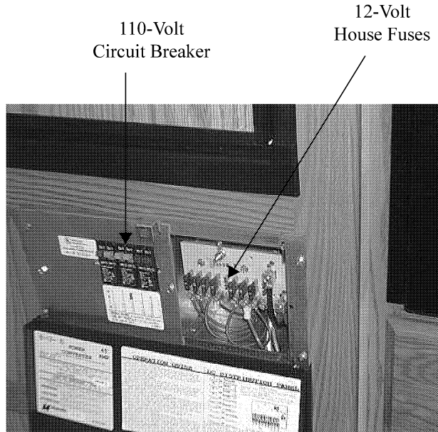
Power Center
