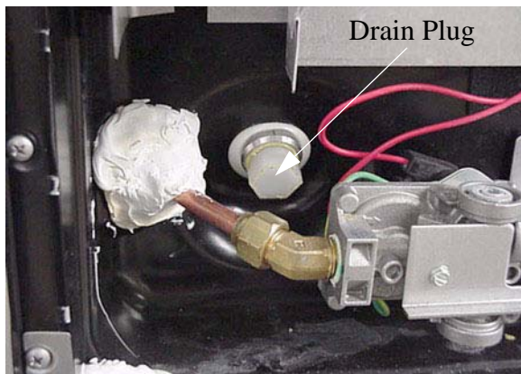
Water Heater Service Access -Typical View
