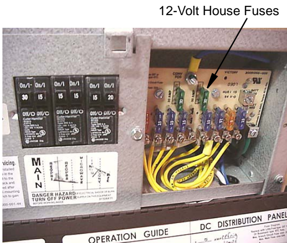
12V Fuse Panel (Located on the right-hand side of the power converter)
