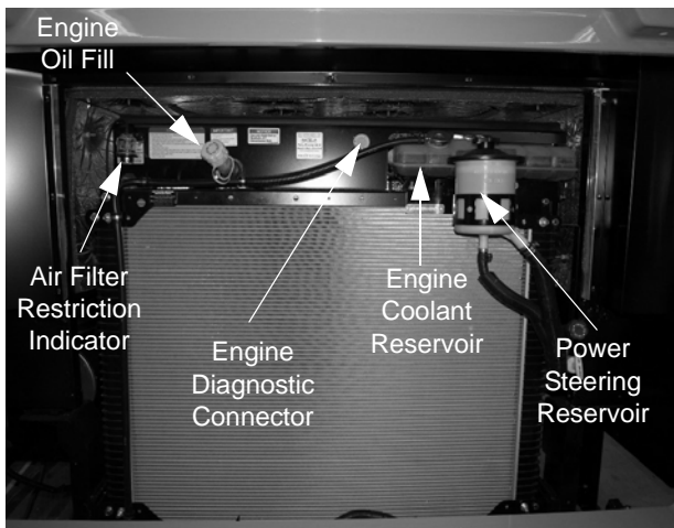
Rear Engine (Shown with grille panel open)
