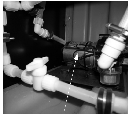
Water Pump (Located in water service center) -Typical View
