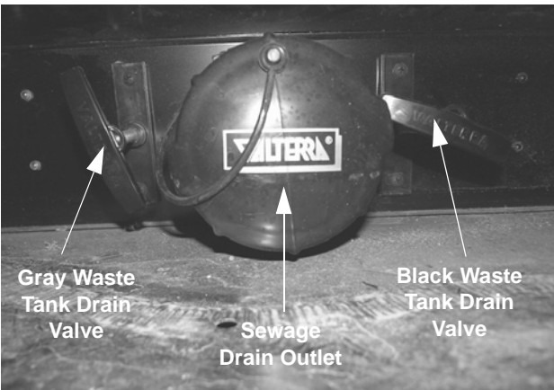
Holding Tank Drain Valves (Located in water service center)
