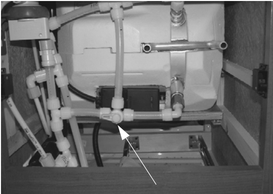
Water Heater Bypass Valve -Typical installation shown
