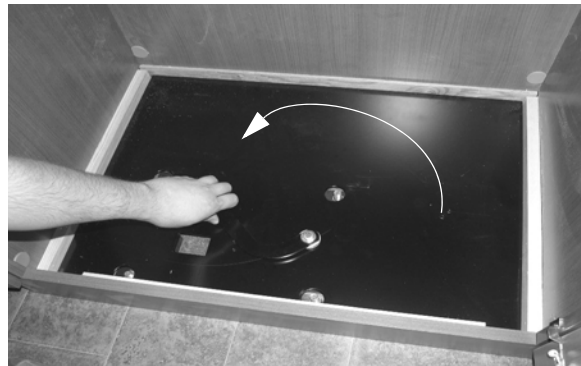
Locking Arm (Located inside Wardrobe Cabinet) - Unlocked position shown
