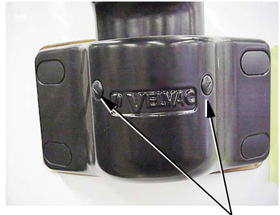
Unscrew protective caps and loosen Allen head set screws to pivot mirror arm. (Torque screws to 75-100 in./lbs.)
