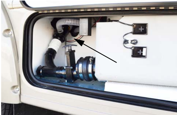
Waste Pump (Located in driver side compartment behind rear wheel)
