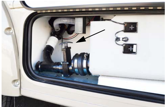
Gray Waste Tank Drain Valve (Located in driver side compartment behind rear wheel)
