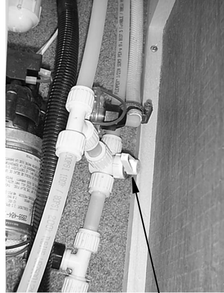
Water Line Drain Valve (Typical)
