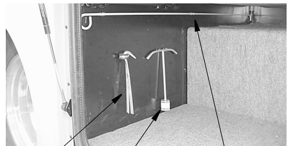
Awning Arm Stake Wheel Liner Tool Awning Hook
