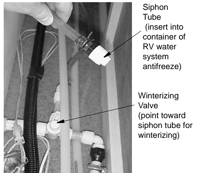
Winterization Valve
