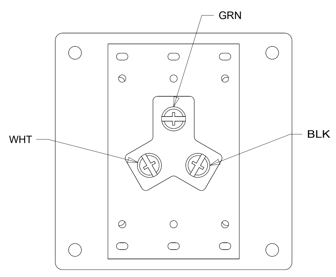
DETAIL AA (BACK VIEW)
